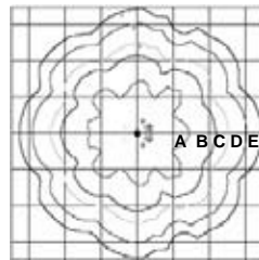
Type V 400w PS VLFG 25ft Mounting Height Foot Candle Key: A=2, B=1, C=.5, D=.2, E=.1 1 Block=30ft
