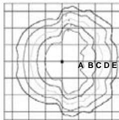
Type III 400w PS VLFG 25ft Mounting Height Foot Candle Key: A=2, B=1, C=.5, D=.2, E=.1 1 Block=30ft
